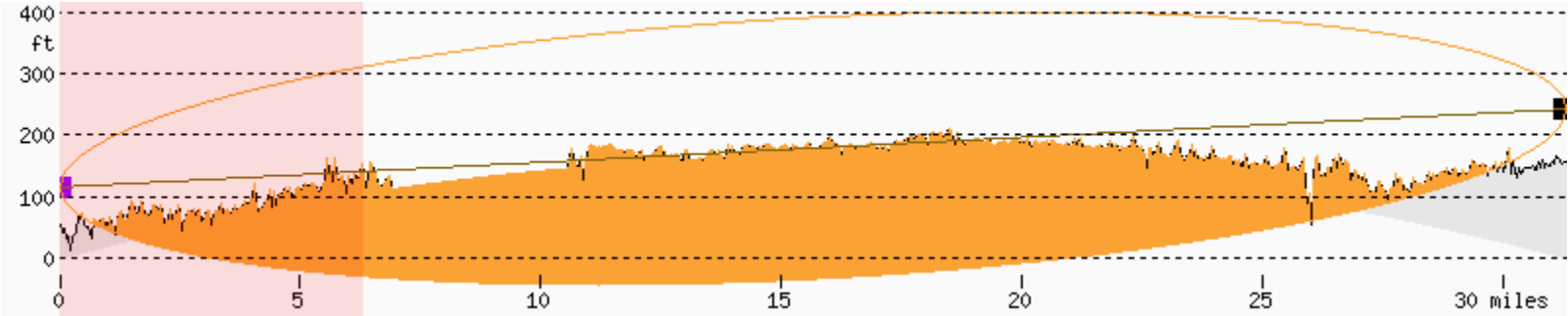
IRVINE 94°0′/31 miles (85 ft above ground, 25 miles range)
