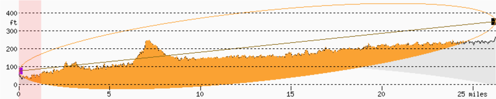
KRAEMER 68°0′/26 miles (85 ft above ground, 25 miles range)
