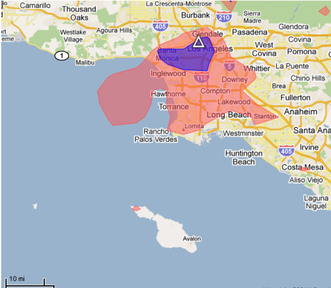
LAMC SUNSET – UHF – 25 WATT – 6DB – PORTABLE COVERAGE
