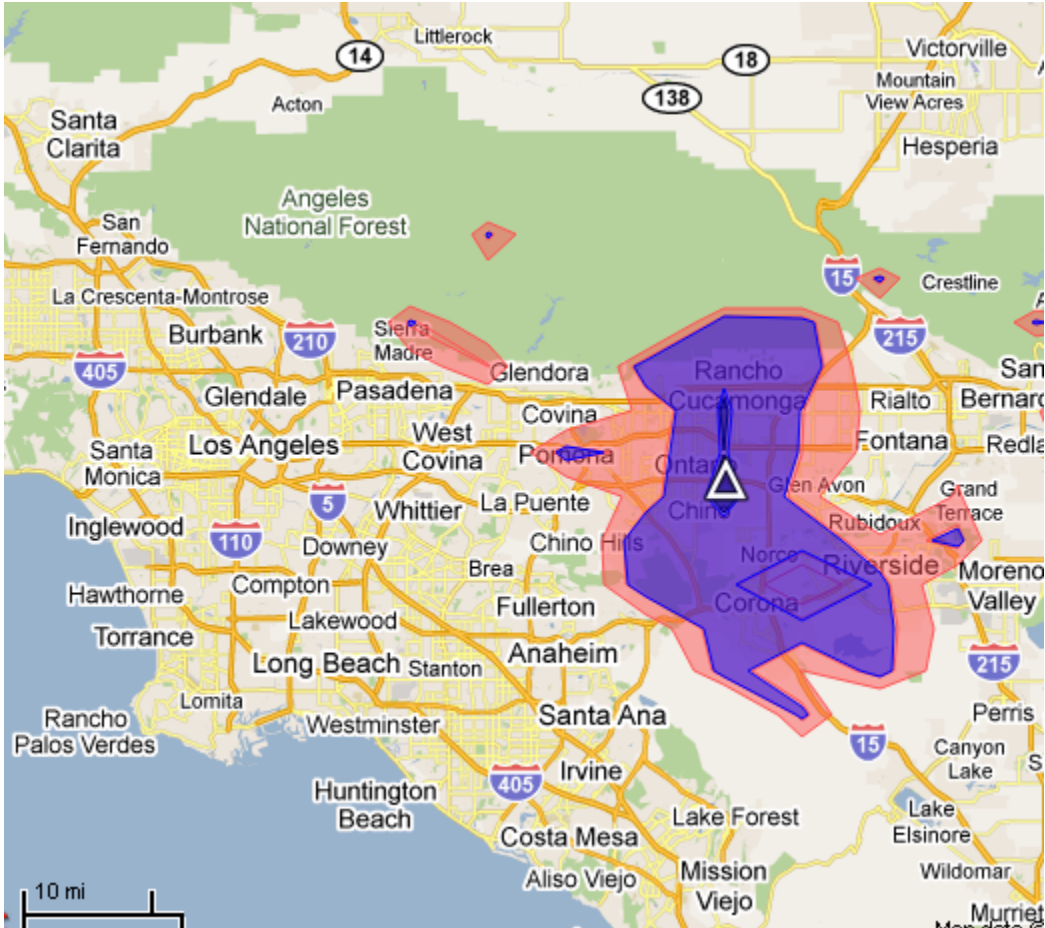
ONTARIO UHF - 25 W - 6DB - PORTABLE COVERAGE
